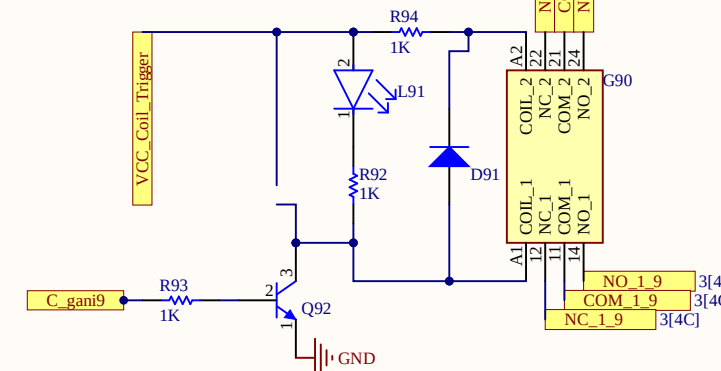
Relay Board
