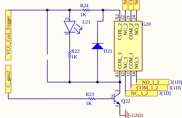
Relay Board
